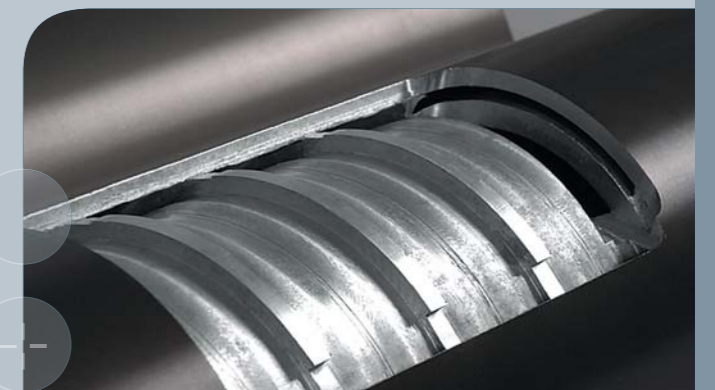
Cross section: cooling roller with internal helix (e.g. cooling rollers for UV dryers, label printing).
